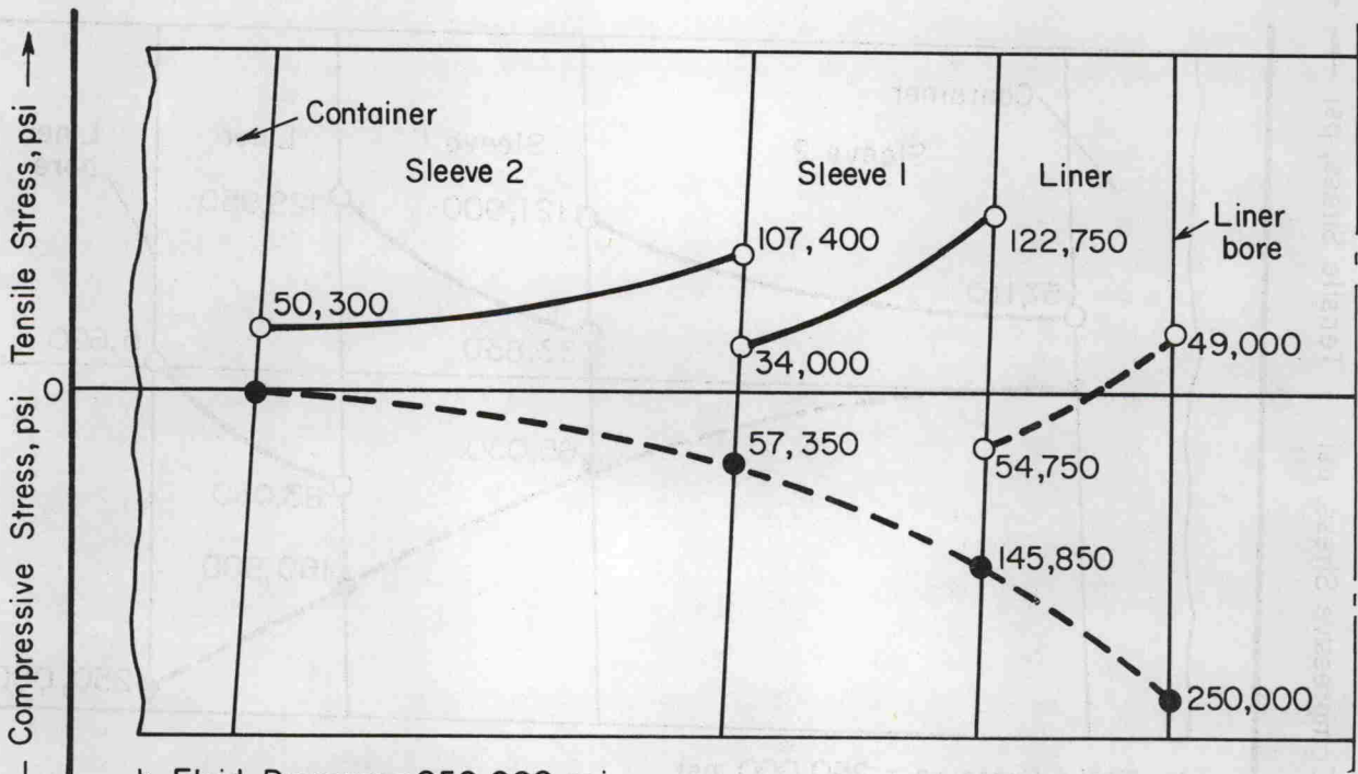
b. Fluid Pressure = 250,000 psi
