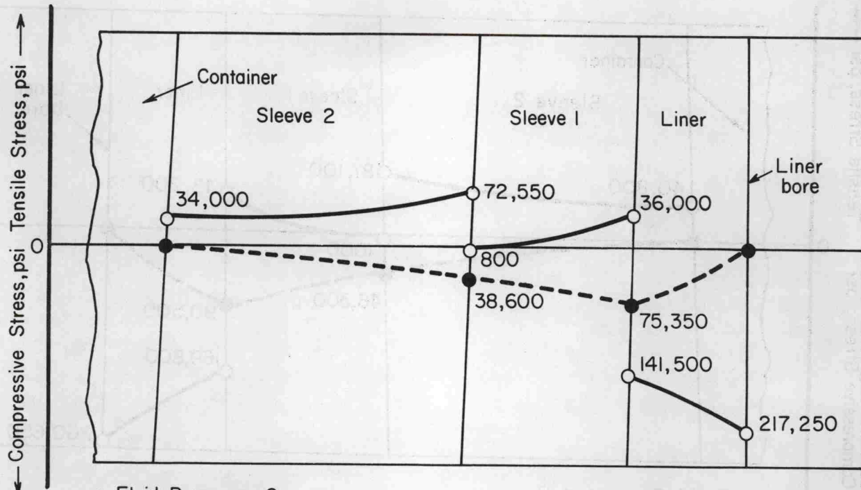
a. Fluid Pressure = 0
